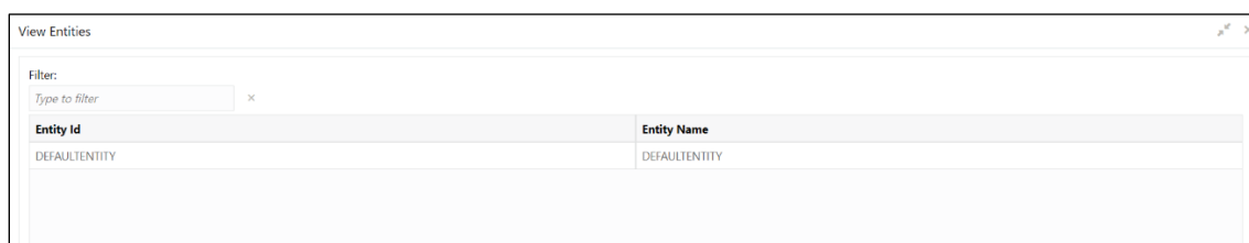
Figure 7: View Entity
