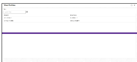
Figure 3: View Entities
