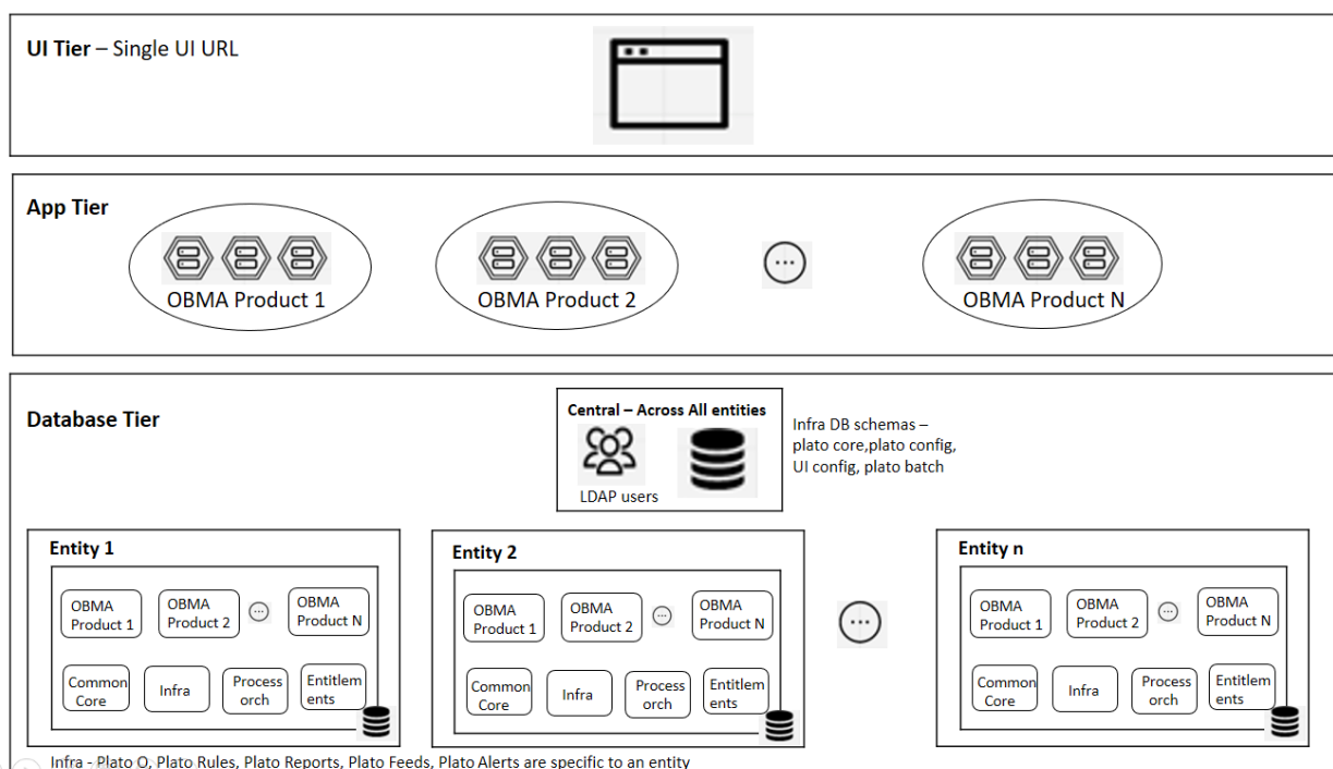
Figure 1: Deployment Diagram.
